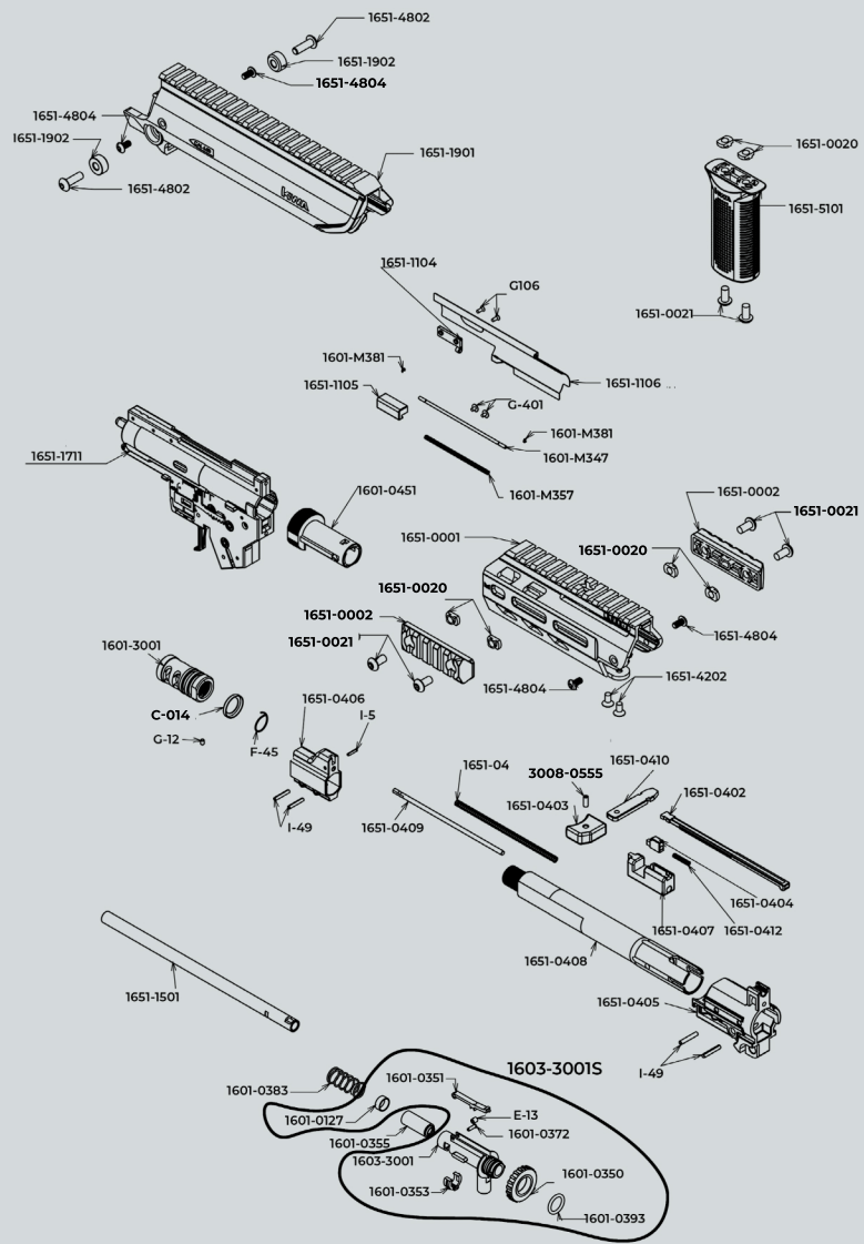
LUCY-4 PARTS
