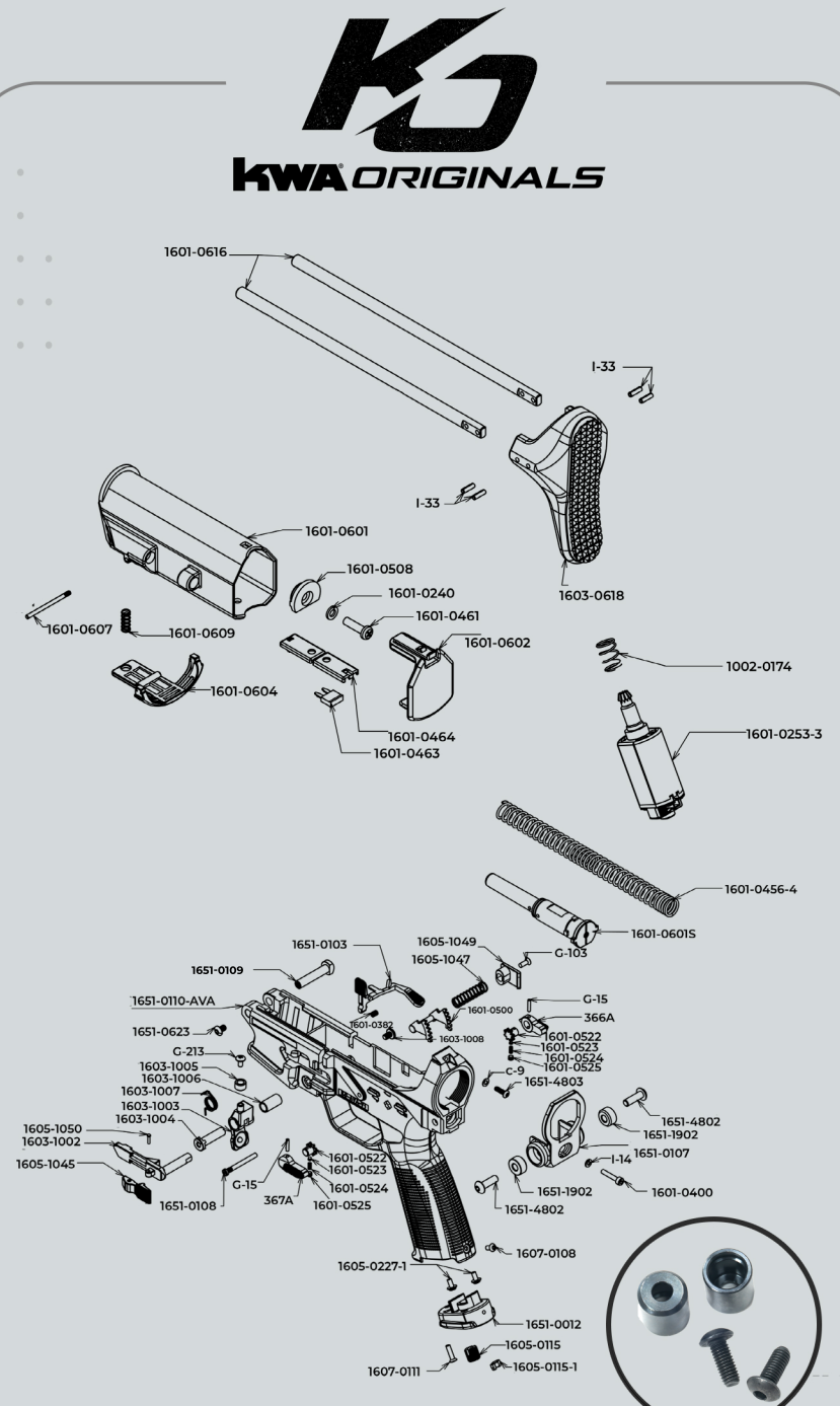
AVA-4 PARTS
