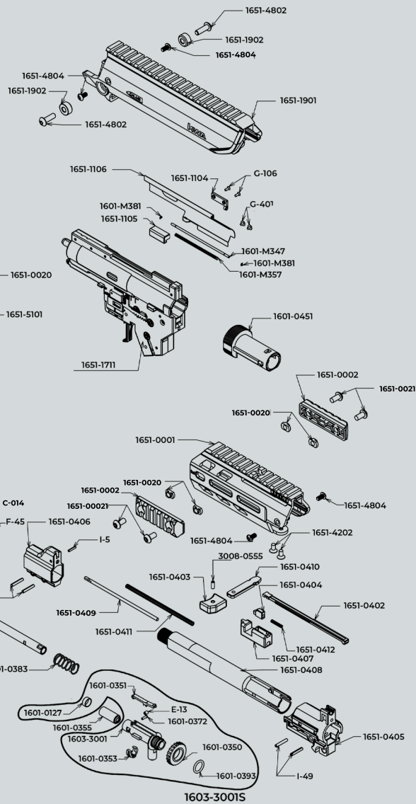
AVA-4 PARTS
